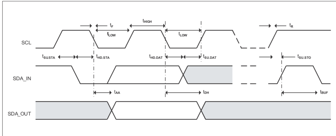
Figure 10: SCL: Serial Clock, SDA: Serial Data I/O
