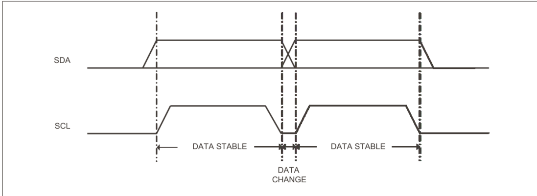
Figure 1: Data Validity
