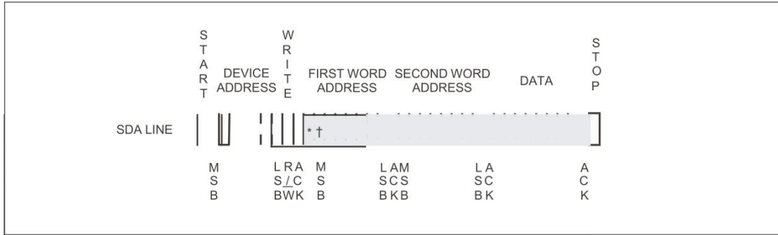
Figure 5: Byte Write
