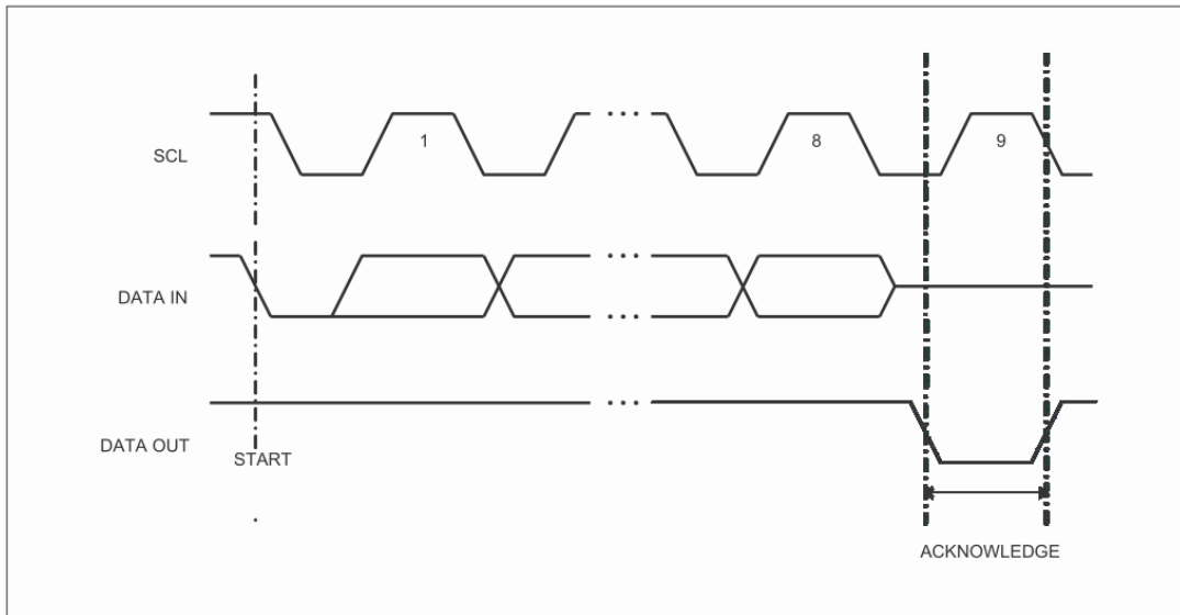
Figure 3: Output Acknowledge
